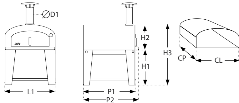
Vista frontale - View from the front
