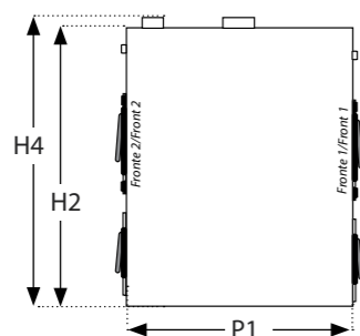
Vista laterale - View from the side
