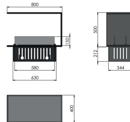
INVAPO INSIDE U 800 800x500x400
