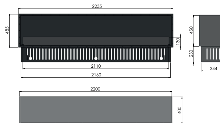
INVAP0 INSIDE 2200 2235x400x485 + 230 (instalation module)
