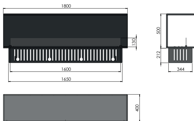
INVAPU INSIDE C 1800 1800x400x500 + 212 (instalation module)
