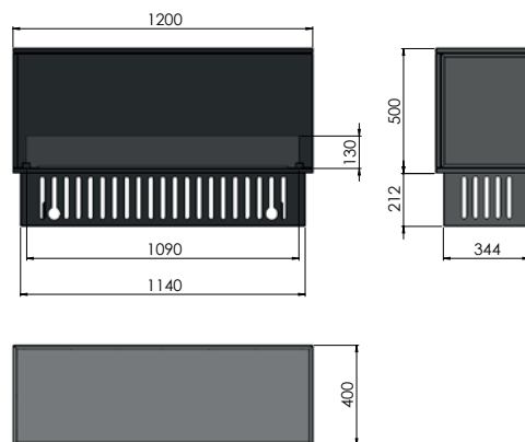
INVAPO CORNER R1200 1200x400x500 + 212 (instalation module)
