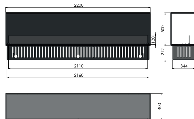
INVAPU INSIDE C 2200 2200x400x500 + 212 (instalation module)
