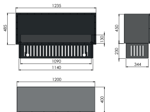
INVAP0 INSIDE 1200 1235x400x485 + 230 (instalation module)
