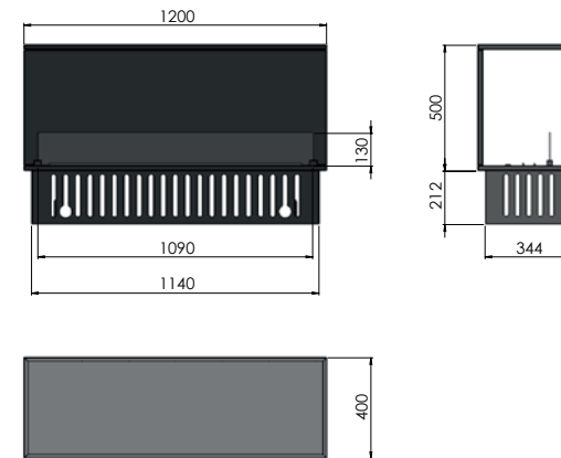
INVAPU INSIDE C 1200 1200x400x500 + 212 (instalation module)
