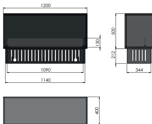
INVAPO CORNER L1200 1200x400x500 + 212 (instalation module)
