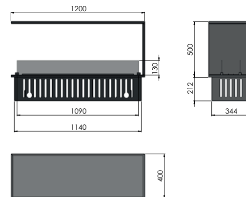
INVAPO INSIDE U 1200 1200x400x500 + 212 (instalation module)
