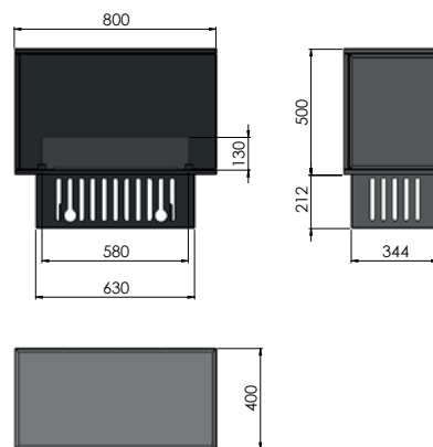
INVAPO CORNER R800 800x400x500 + 212 (instalation module)
