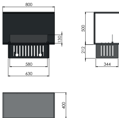
INVAPU INSIDE C 800 800x400x500 + 212 (instalation module)
