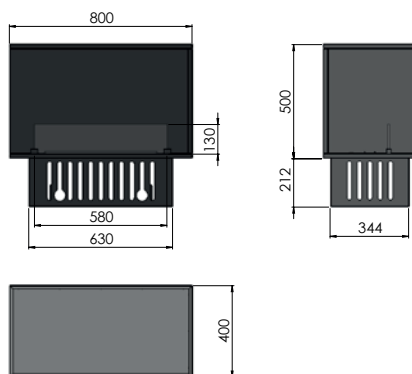
INVAPO CORNER L800 800x400x500 + 212 (instalation module)
