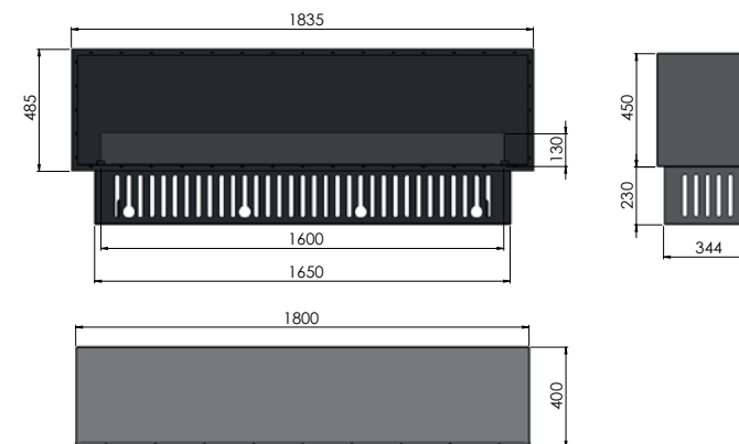
INVAP0 INSIDE 1800 1835x400x485 + 230 (instalation module)
