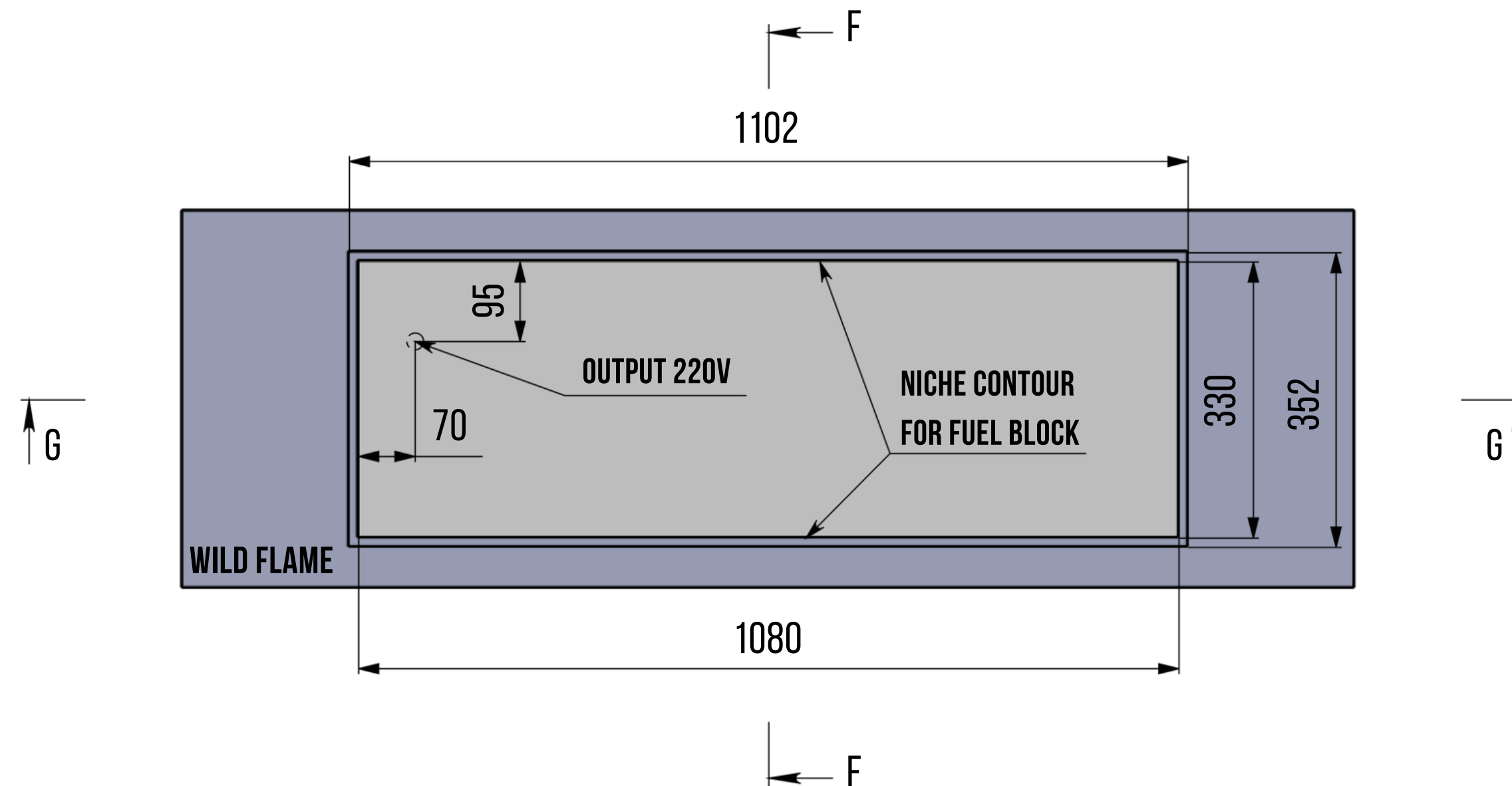
FRONT VIEW
