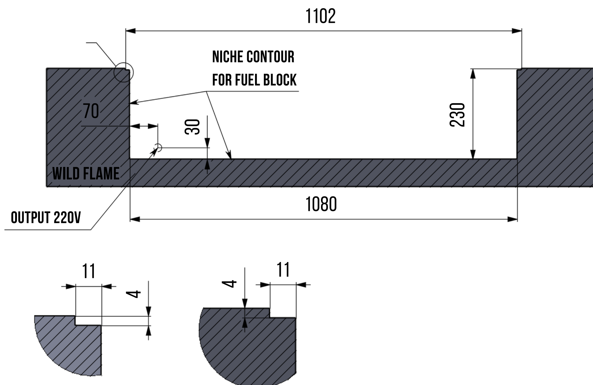
FRONT VIEW
